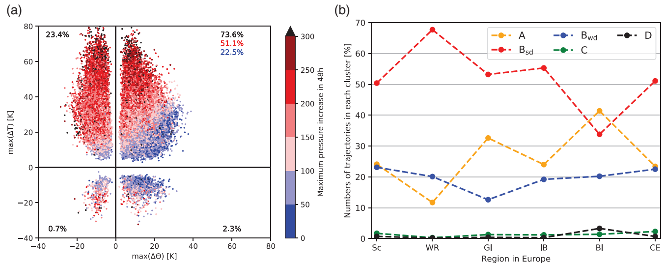
FIGURE 6 Thermodynamic changes for the trajectory clusters. (a) Maximum temperature ( \Delta T_{\max} , in K) and maximum potential temperature ( \Delta \theta_{\max} , in K) changes along the trajectories for heat waves in Central Europe. The colours indicate the maximum pressure increase in a 48-hr window. The numbers in the quadrants denote the fraction of trajectories in each cluster: in black (irrespective of descent rate), blue (descent \leq 100 hPa in 48 hr, only upper right quadrant), and red (descent > 100 hPa in 48 hr, only upper right quadrant). Additionally, the letters in boxes indicate the names of the clusters and the black sloping line denotes the approximate border between clusters B_{sd} and B_{wd} . (b) Fraction of trajectories in clusters for all investigated regions in Europe (Sc: Scandinavia, WR: western Russia, GI: Greece/Italy, IB: Iberian Peninsula, BI: British Isles, CE: Central Europe)
